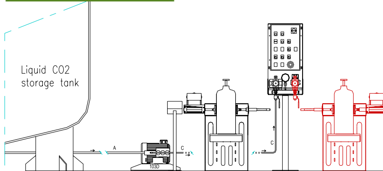
Front view of an installed complete station
