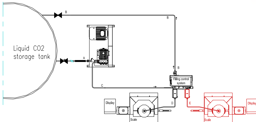
Complete lay-out
